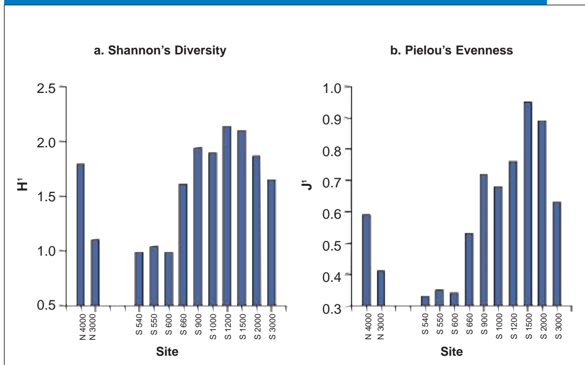
Figure 3.10. Comparison of infaunal diversity and evenness between sites (NW to SE of outfall).
