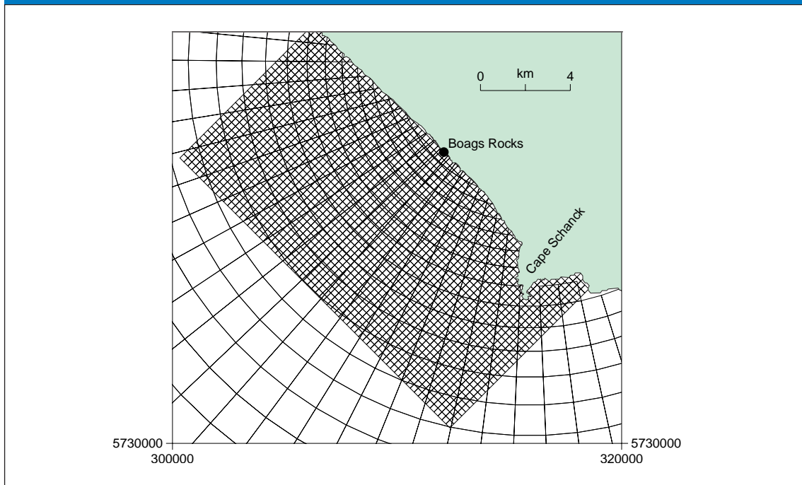
Figure 3.15. Rectangular grid overlayed on the polar grid covering Bass Strait.
