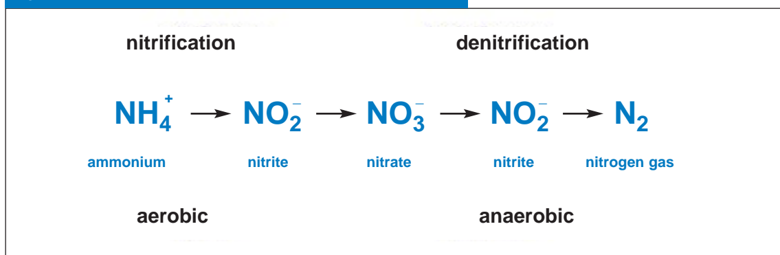
Figure 3.18. Chemical process for nitrification/denitrification
