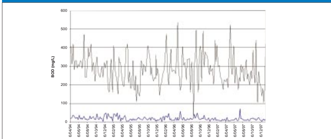
Figure 2.3. BOD of the untreated sewage (higher line) and BOD of the treated effluent (lower line) for ETP.
