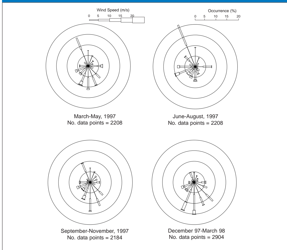
Figure 2.7. Telescope plots of wind data measured at Gunnamatta Surf Life Saving Club for each of the modelling periods. The telescopes point towards the directions from which the wind is blowing, the width of the scope indicates wind speed and the length indicates percentage of time they occur (Andrewartha et al. 1998).
