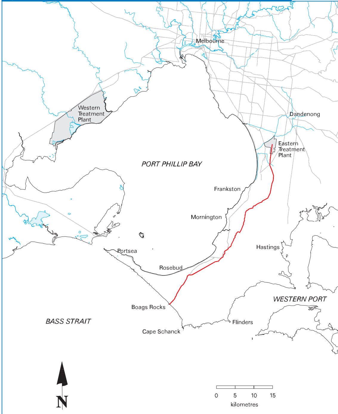
Figure 2.1. Location of Eastern Treatment Plant, with ocean outfall to Boags Rocks
