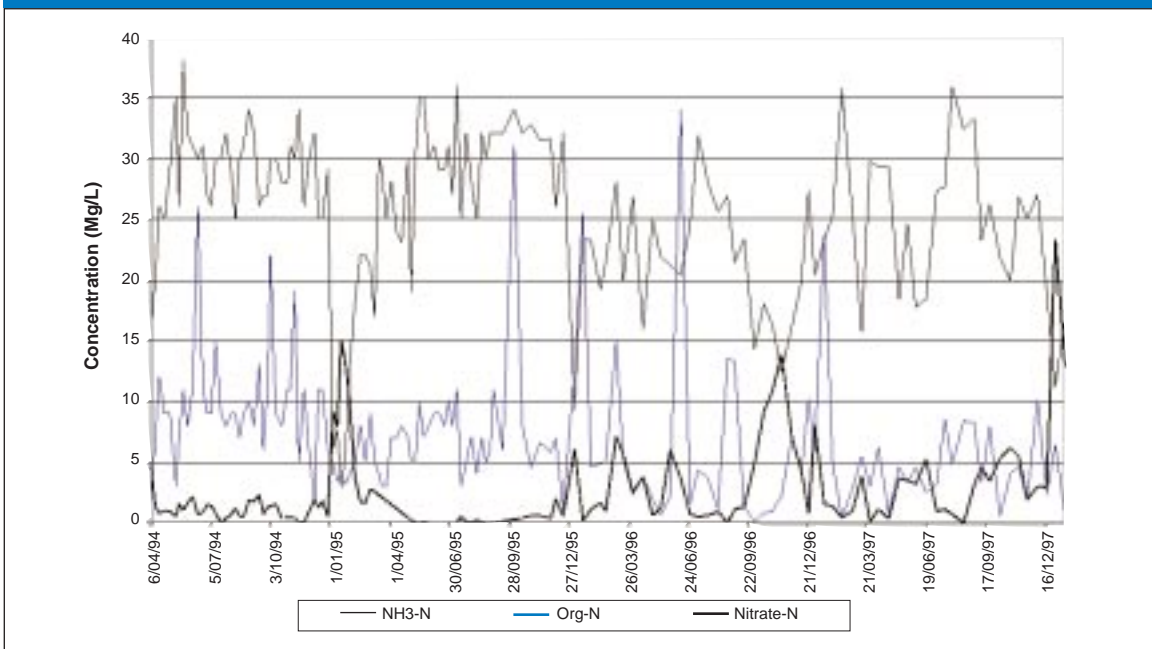
Figure 2.5. Nitrogen in the form of ammonia (higher line), organic nitrogen (middle line) and nitrate (lowest line) from fortnightly samples of treated ETP effluent.
