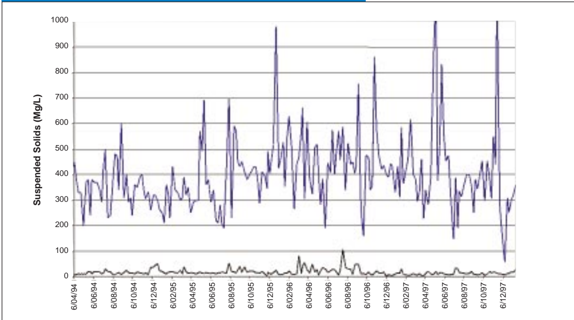
Figure 2.4. Suspended solids in the untreated sewage (higher line) and in the treated effluent (lower line) for ETP.
