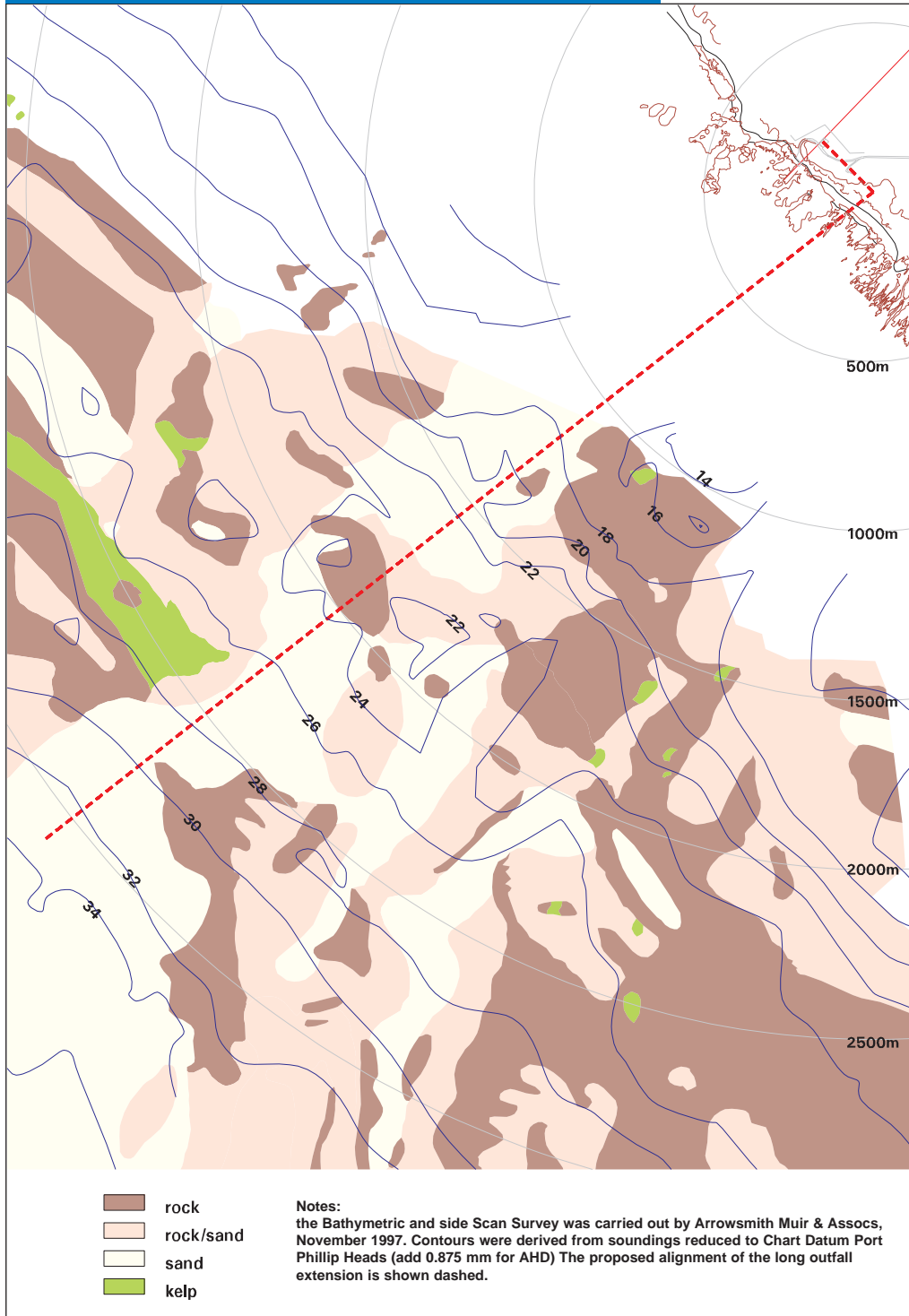
Figure 3.16. The path proposed by CEE for extending the outfall.
